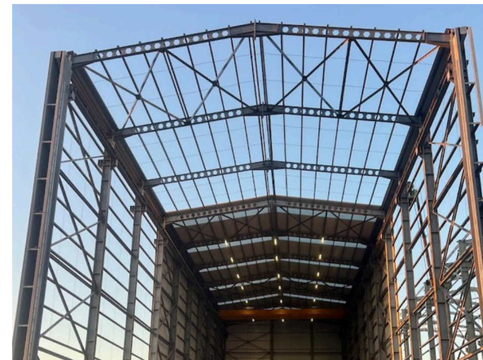
STEEL CONSTRUCTION
